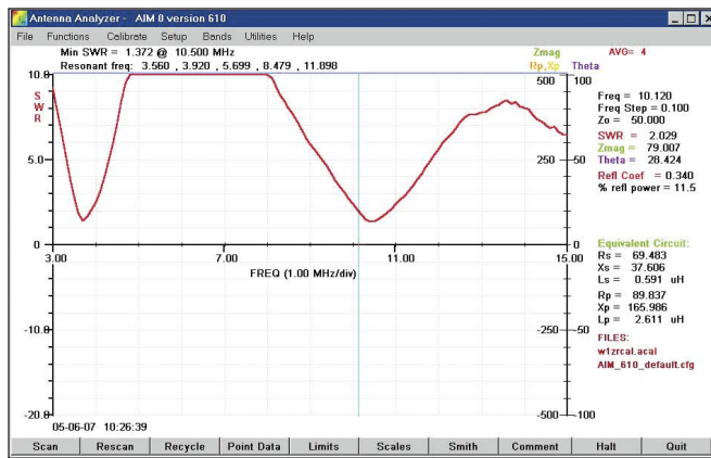
Figure 2 — AIM4170 output with just an SWR plot. Seems a bit easier to grasp.
