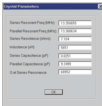
Figure 4 — AIM4170 output while measuring crystal parameters.
