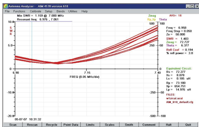
Figure 3 — Family of curves as I adjusted my tuner for an SWR of less than 2:1 over the 40 meter CW segment.
