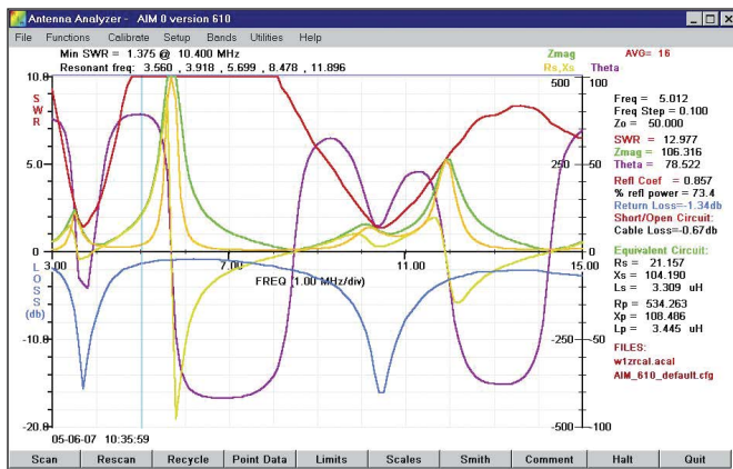
Figure 1 — AIM4170 default output with plots of almost all possible outputs in living color.
