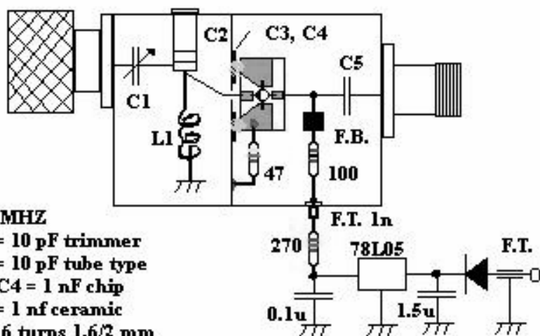
Bird view of the tiny box
