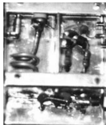
Enlarged view of 432 Mhz preamp
